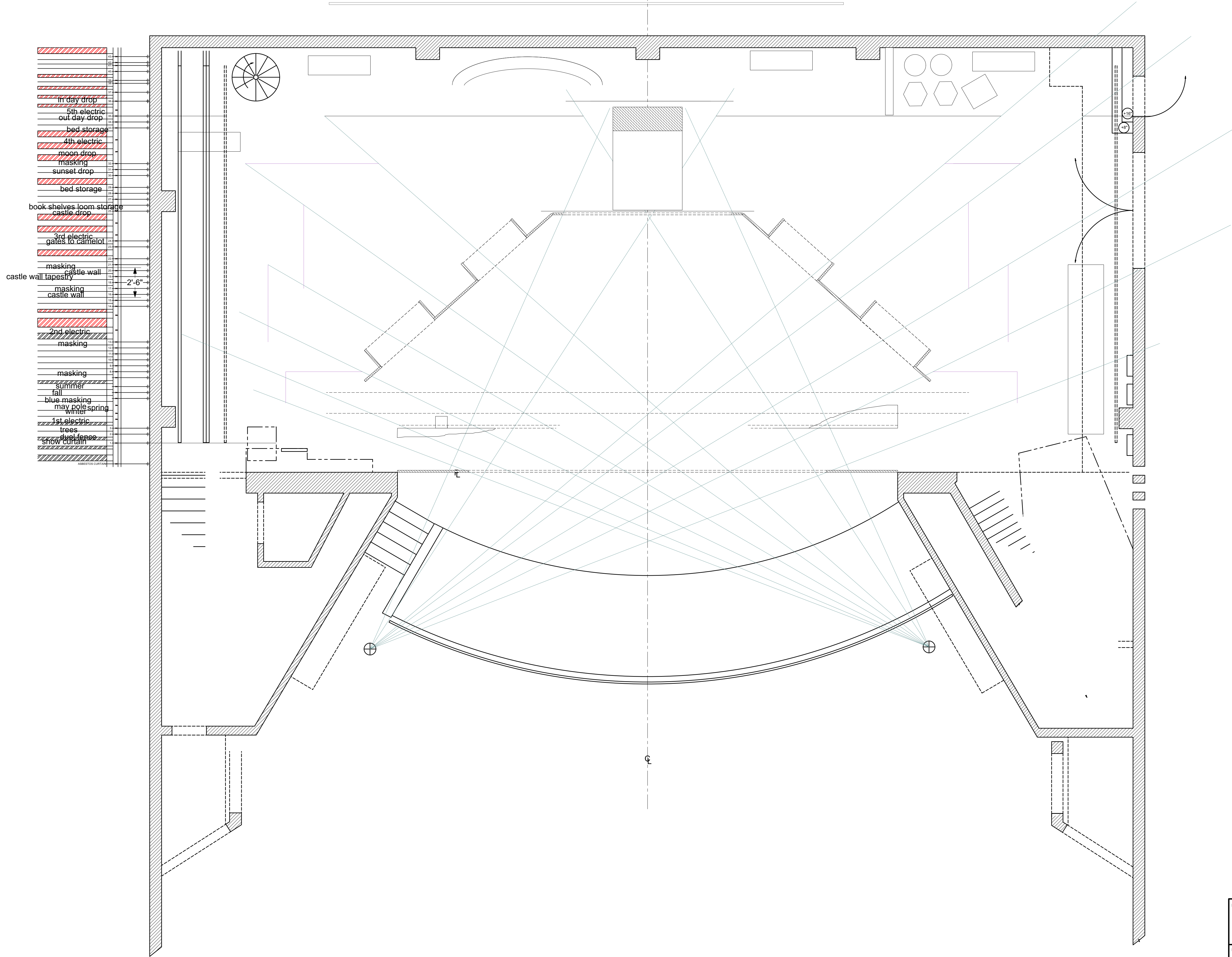
11 Act 2 Scene 4 Scale: 1/4" = 1'-0"
