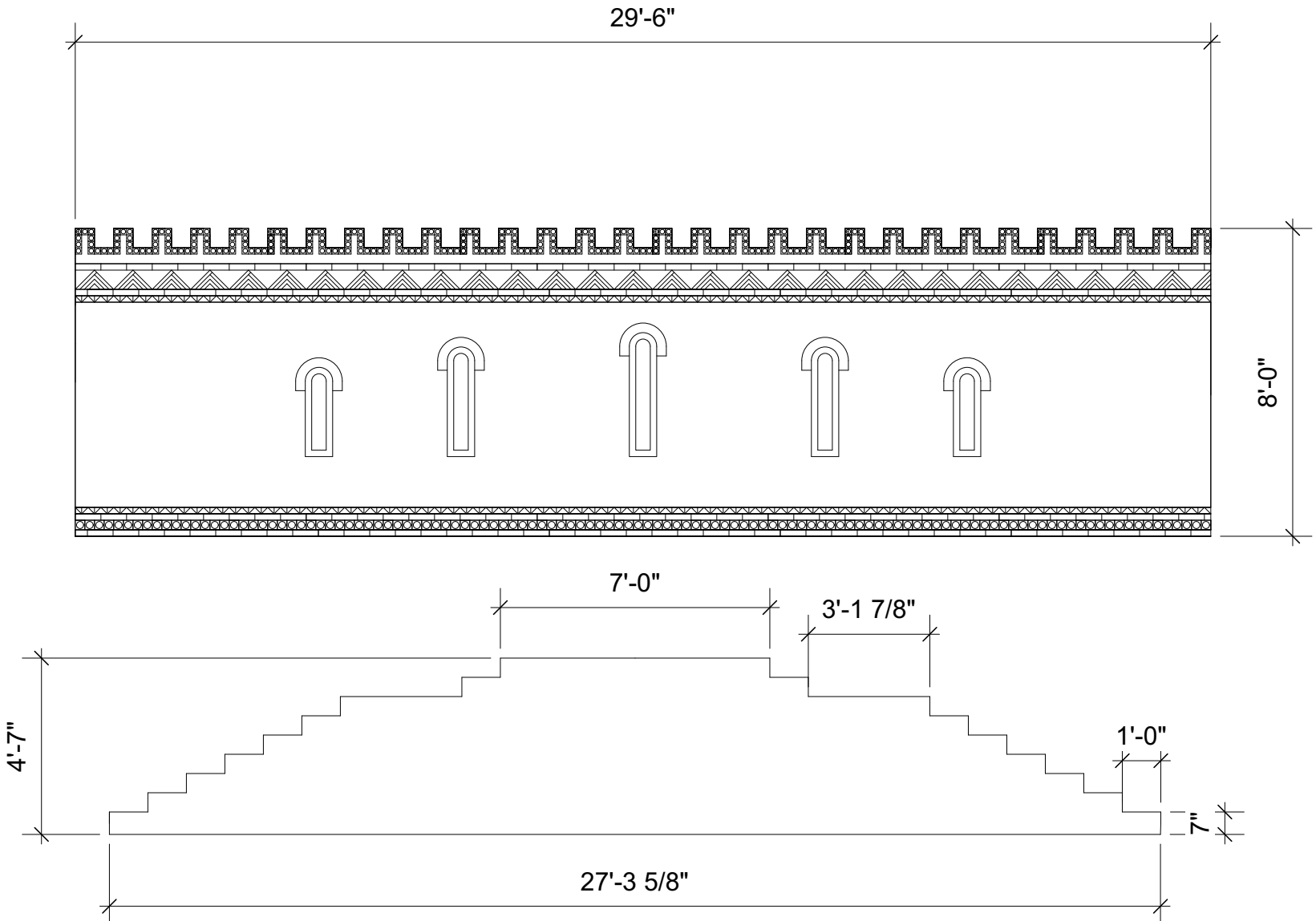
16.3 Wall Stairs Scale: 1/4" = 1'-0"
