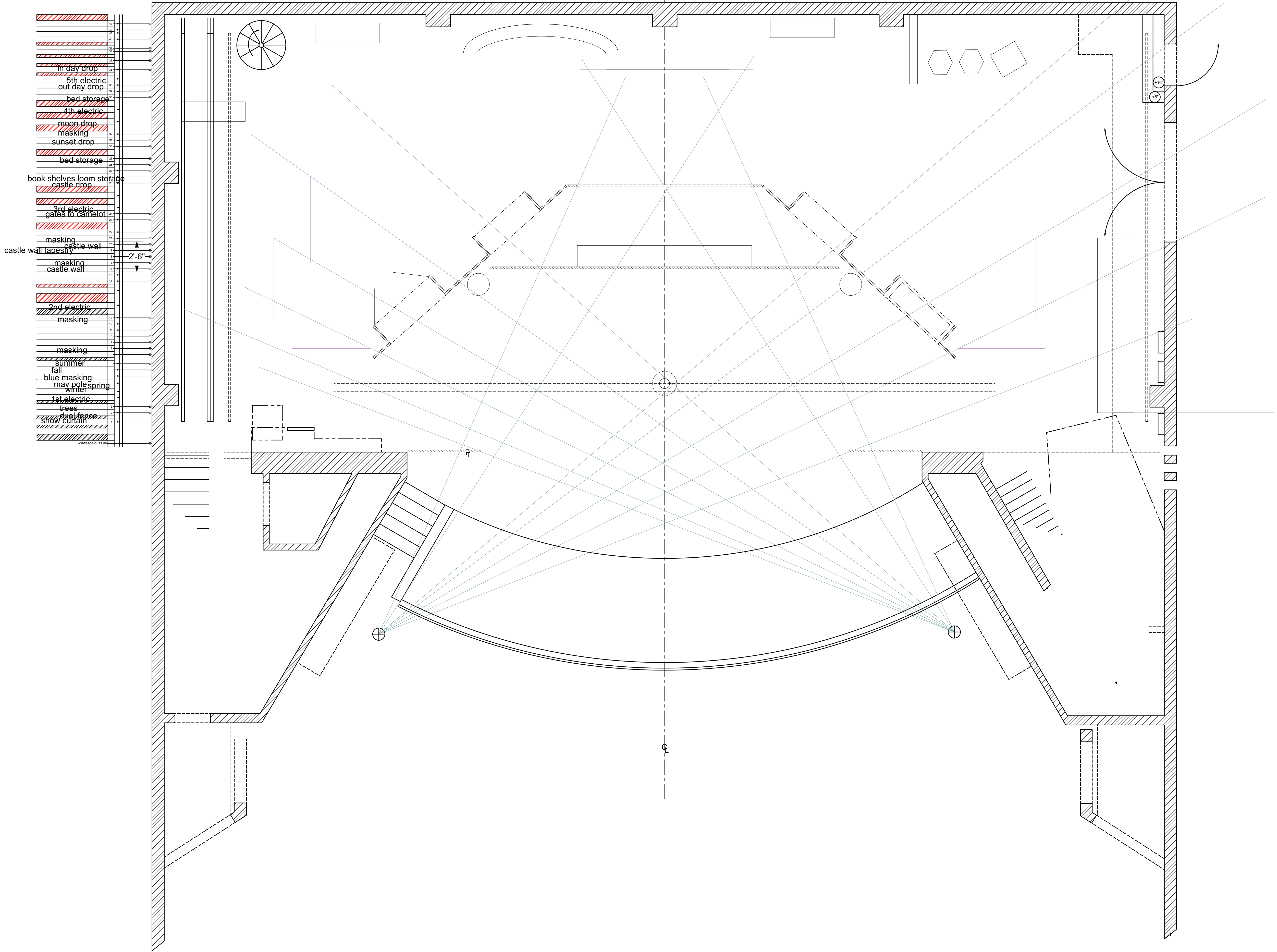
6 Act 1 Scene 4 Scale: 1/4" = 1'-0"
